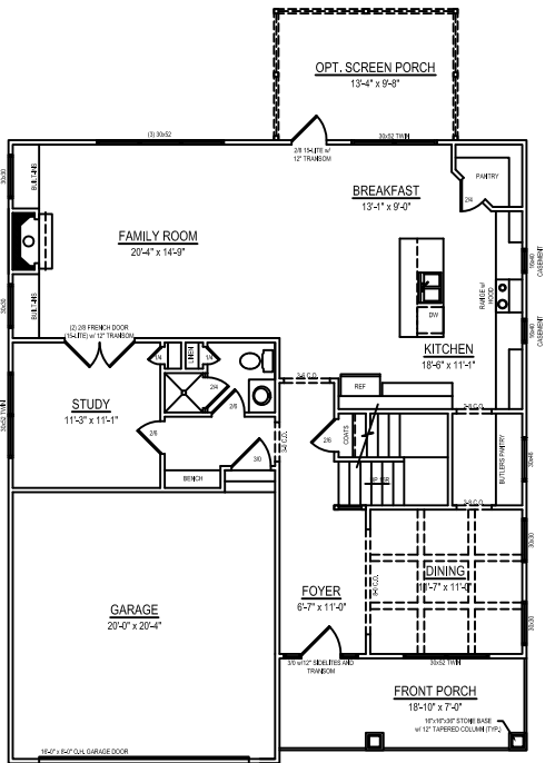
FIRST FLOOR PLAN CEILING HT. = 9'-0"
