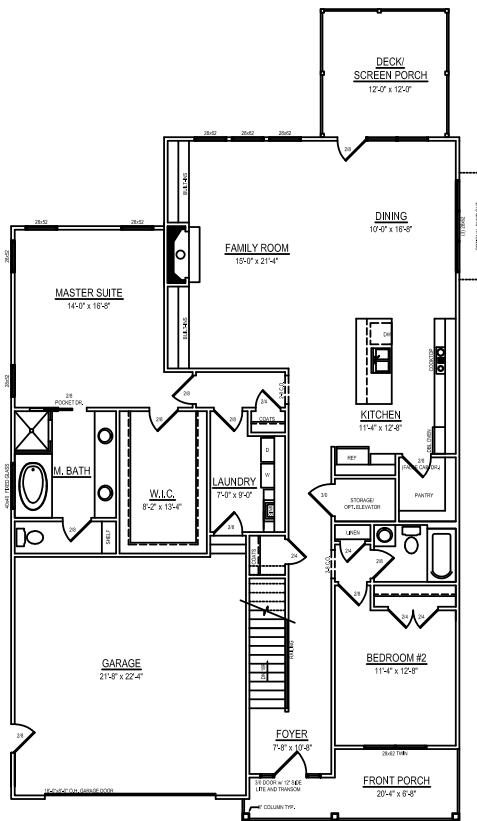
FIRST FLOOR PLAN CEILING HT. = 10'-0"
