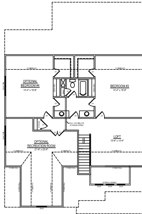
SECOND FLOOR PLAN CEILING HT. = 8'-0"
